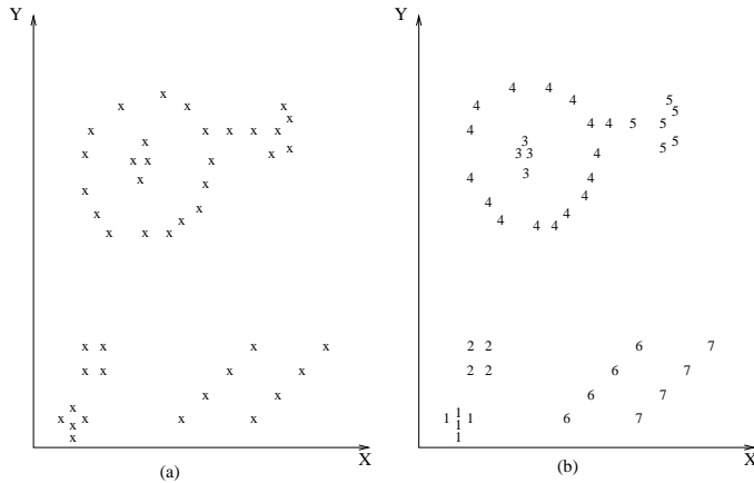
Figure 1. Data clustering.
