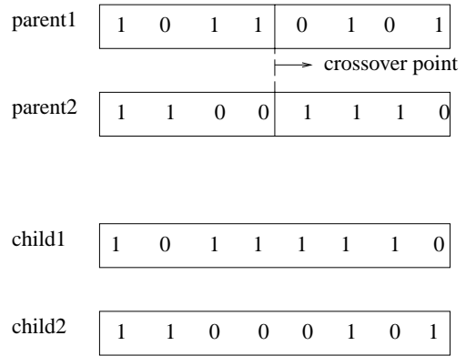
Figure 20. Crossover operation.
